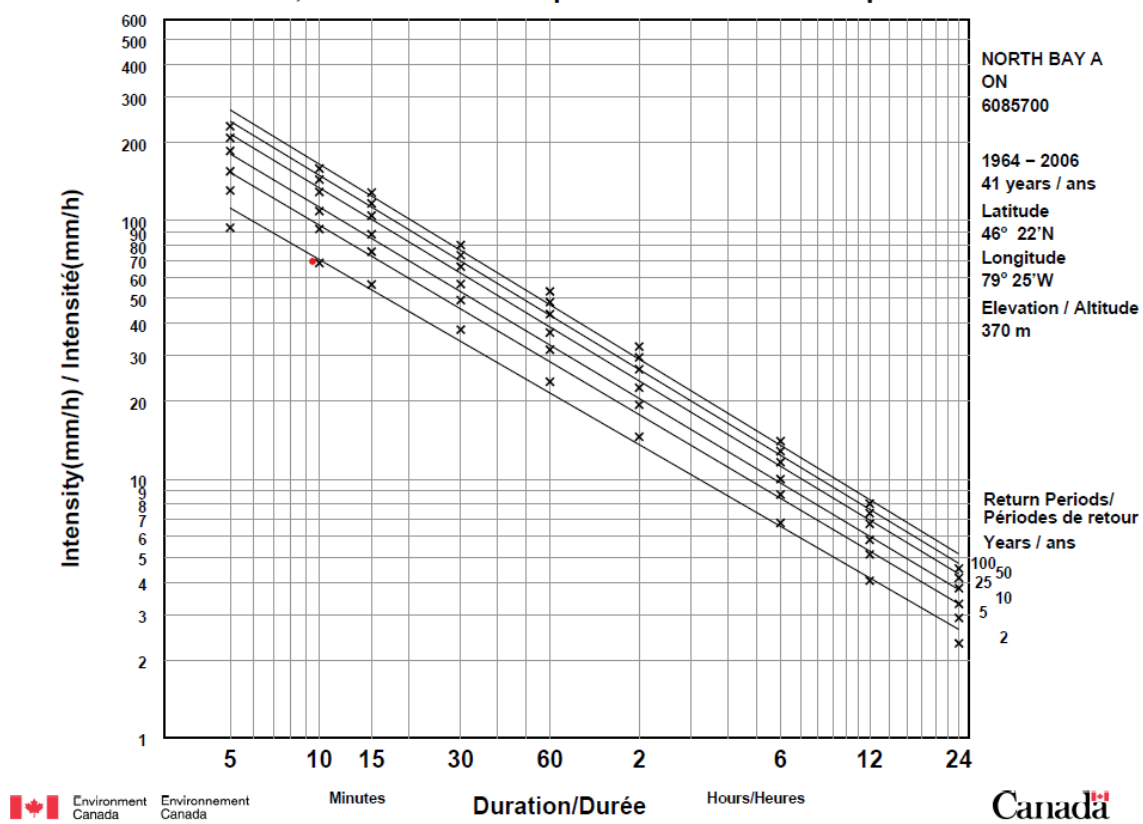
Figure 10.7 Short Duration Rainfall Intensity-Duration-Frequency Data (Environment Canada, 2019/02/27)
